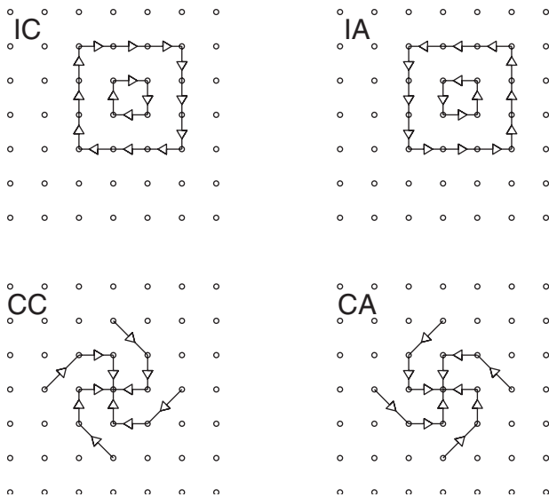
Fig. 2. Four vortices
