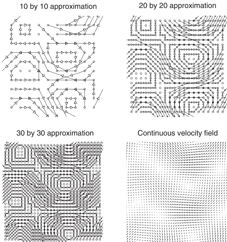
Fig. 1. Discrete approximations of a continuous velocity field
